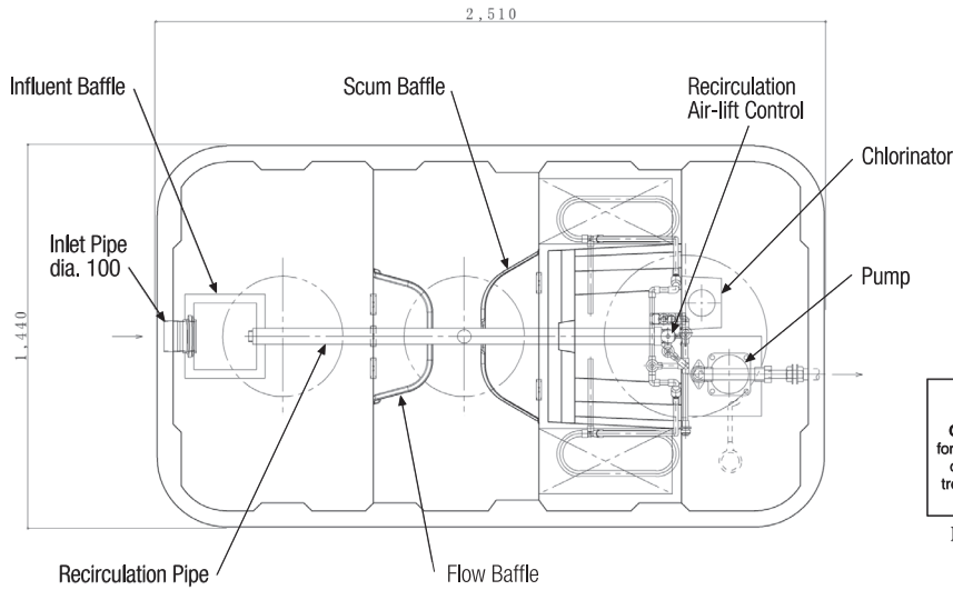
Horizontal Sectional View
