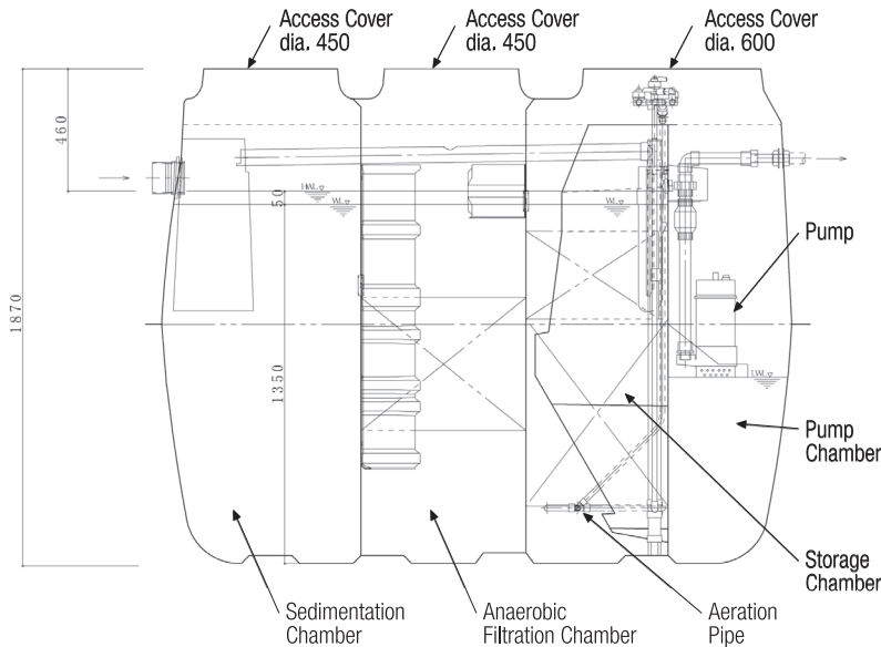
Vertical Sectional Views
